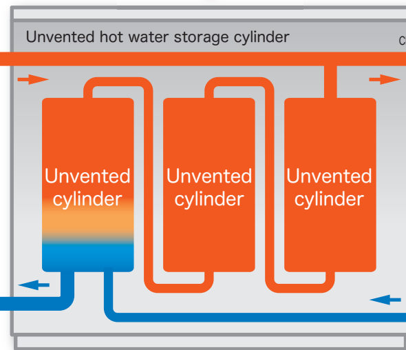
Unvented cylinder
